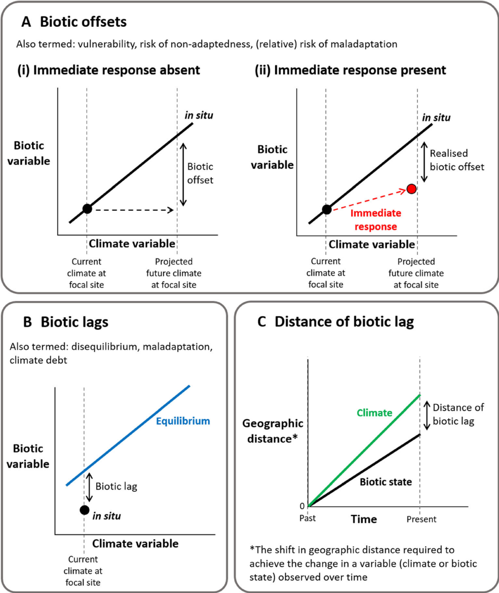
Fig. 3. Space-for-time substitution (SFTS) metrics predicting the challenge that climate change poses to aspects of biodiversity. Black circles represent a focal site. (A) Biotic offset, the distance between the current biotic state at a focal site and the predicted equilibrium biotic state at that site under future climate conditions. The current biotic state may either be (i) that observed in situ at the focal site or (ii) that accounting for an immediate biotic response to climate change (e.g. due to phenotypic plasticity; red circle) which can be observed via a transplant experiment representing the expected future conditions (realised biotic offset). (B) Biotic lag, the distance between the observed biotic state at a focal site and the predicted equilibrium biotic state at that site under current climatic conditions. (C) Where both spatial and temporal data are available, temporal shifts in both biotic states and climate variables can be quantified in terms of an equivalent shift in spatial distance, and this can be used to find the distance of biotic lag. Linear climate–biotic relationships are depicted here for simplicity but some relationships may be non-linear. Note that where the biotic response is a species’ distribution, the focus is generally on how the biotic state (presence or abundance) covaries with climate across many populations, rather than a single population as depicted here. Where the biotic response is species occurrence, the biotic state can be thought of as either the probability of presence or the climate suitability.
